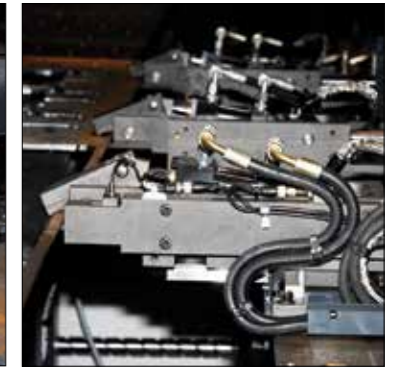
Material clamps
